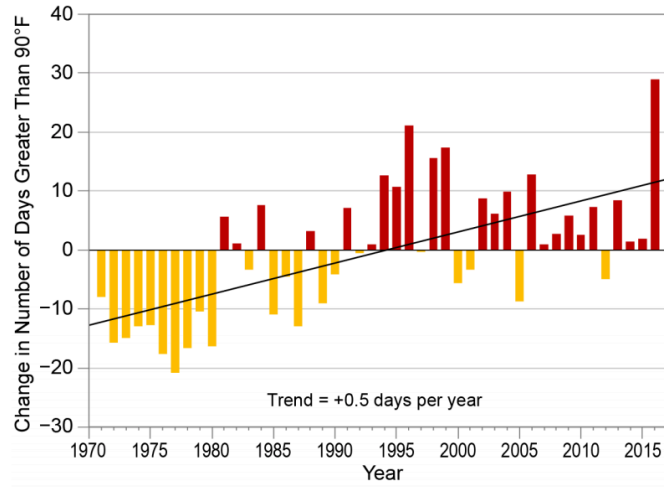
Figure 20.14: This figure illustrates the deviation from the long-term (1971–2016) average annual number of days exceeding 90°F, based on data from eight climate stations in Puerto Rico. Source: University of Puerto Rico. This caption was revised in June 2019. See Errata for details: https://nca2018.globalchange.gov/downloads
