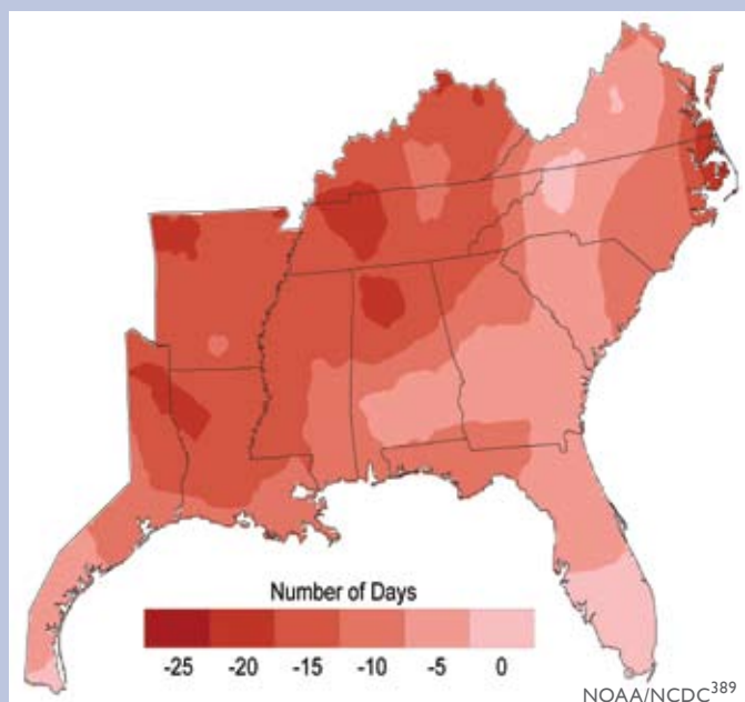
Change in Freezing Days per Year 1976 to 2007
